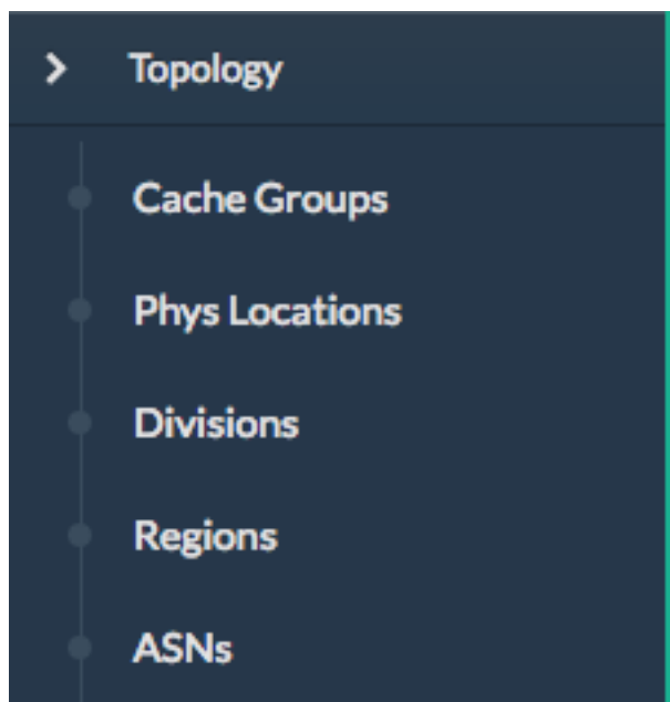
Fig. 17: ‘Topology’ Menu
