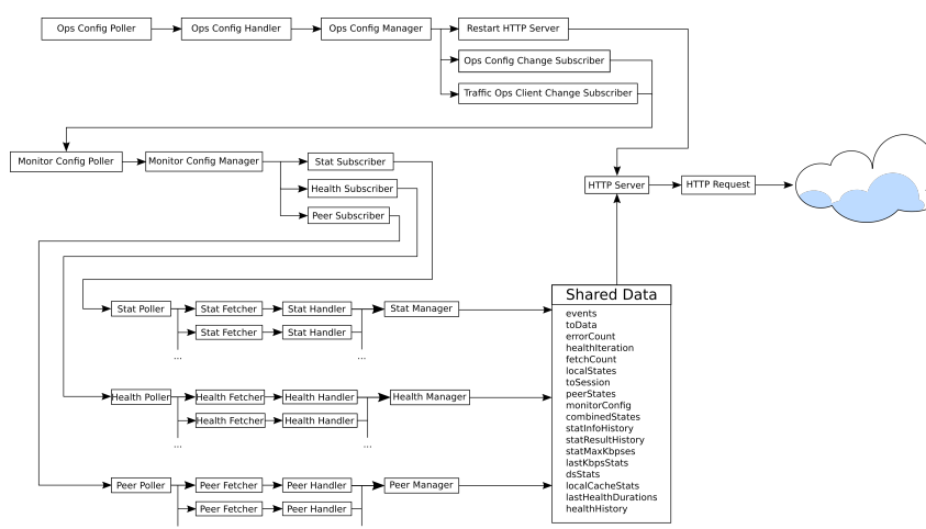
Fig. 50: Pipeline Overview
