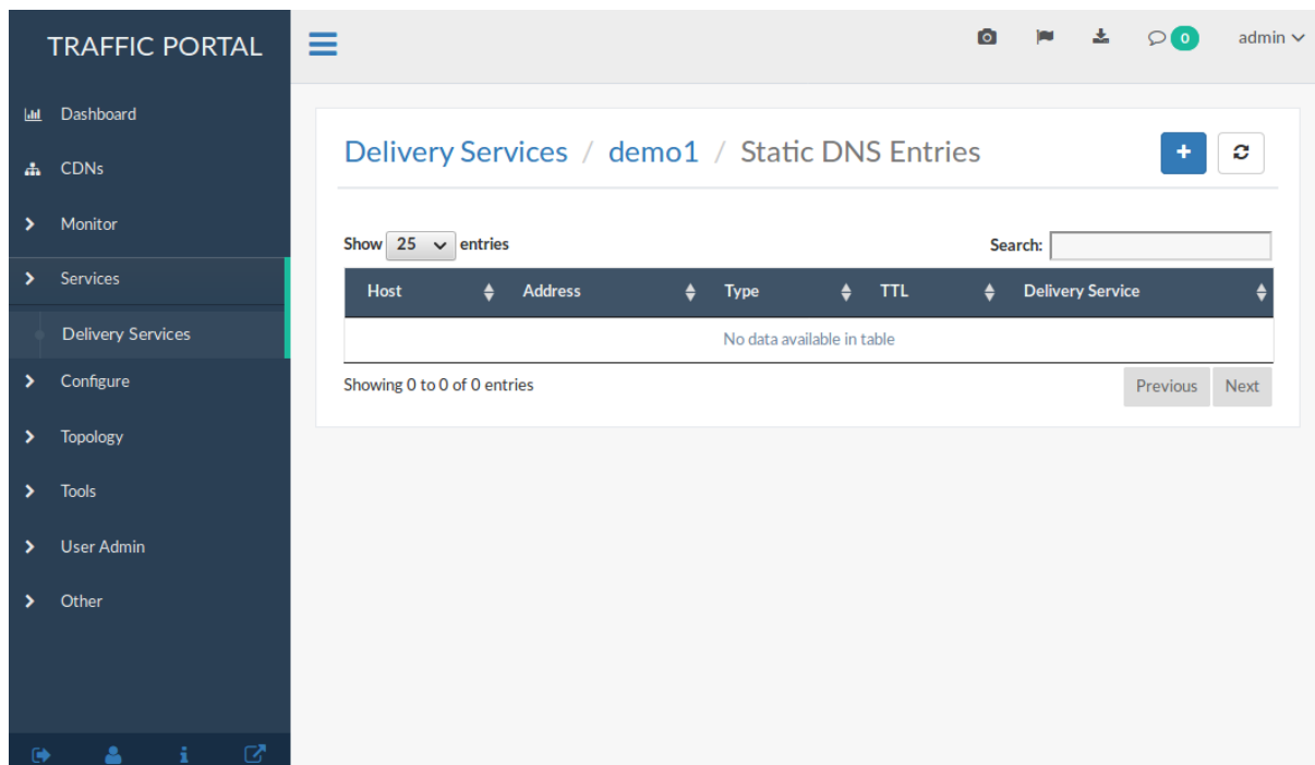
Fig. 45: The Static DNS Entries Table Page
