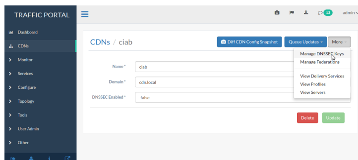
Fig. 32: CDN Details Page
