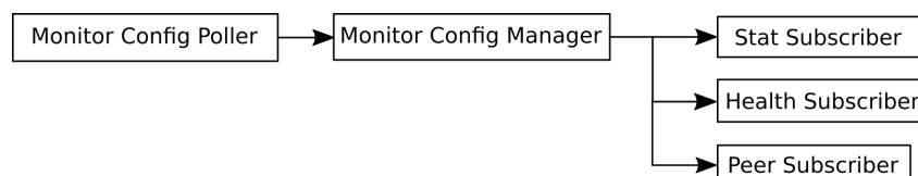
Fig. 54: The Monitor Configuration Pipeline
