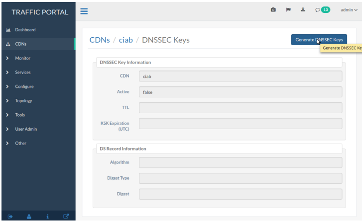
Fig. 33: DNSSEC Key Management Page
