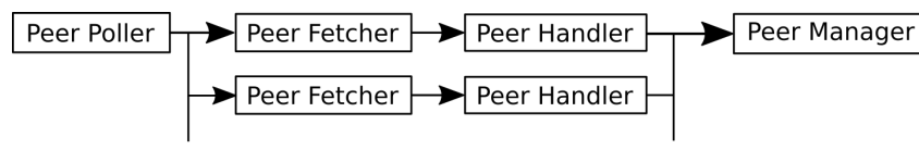
Fig. 53: The Peers Pipeline
