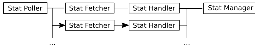
Fig. 51: The Stats Pipeline
